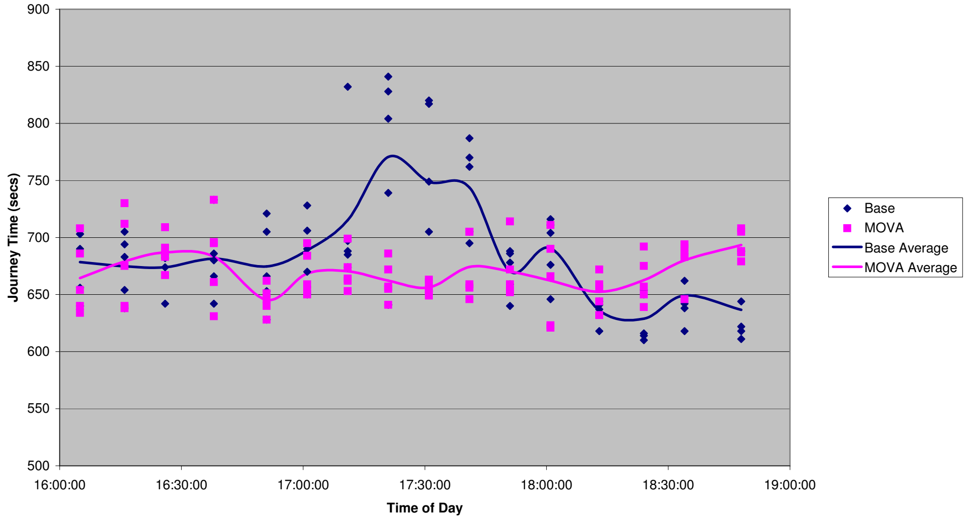
X 78 nb Evening Journey Time Variability - Base compared to MOVA control
