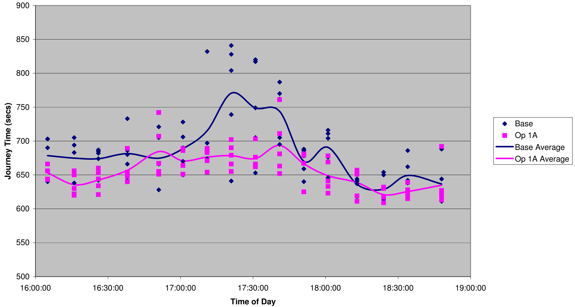
X 78 nb Evening Journey Time Variability - Base compared to Op 1A
