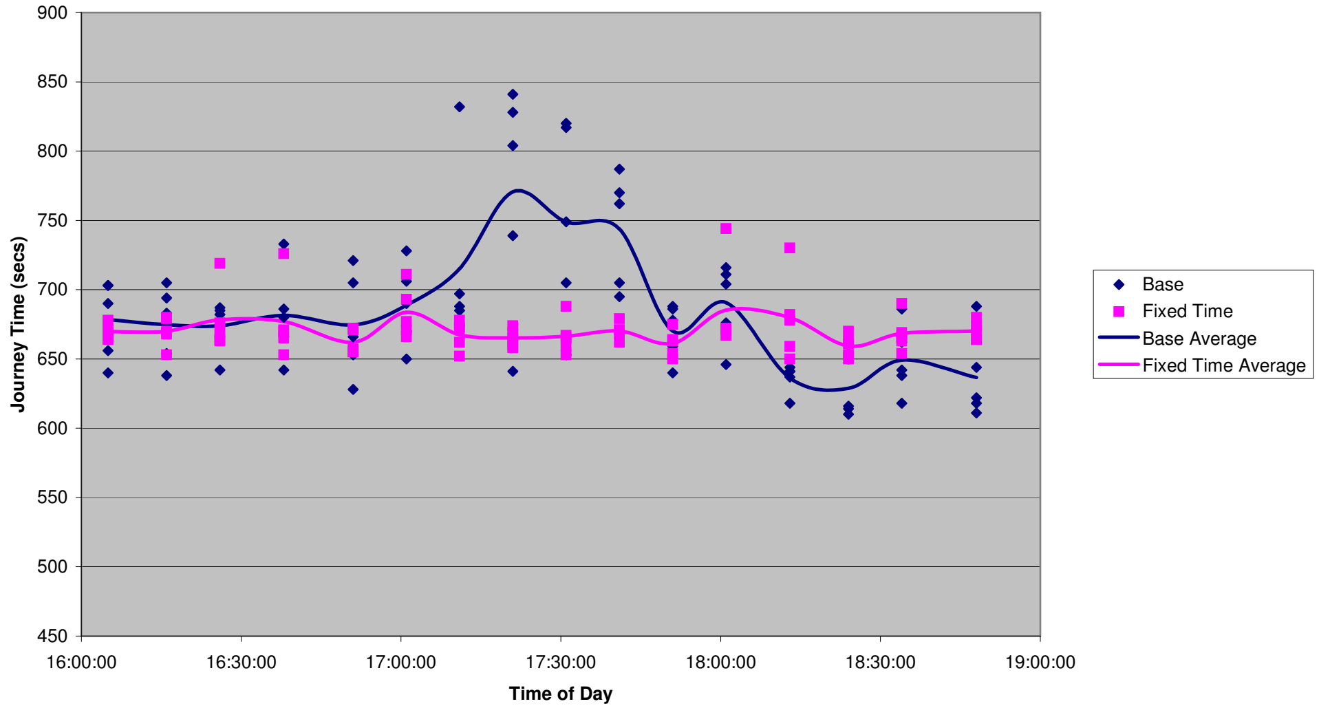
X 78 nb Evening Journey Time Variability - Base compared to Fixed Time
