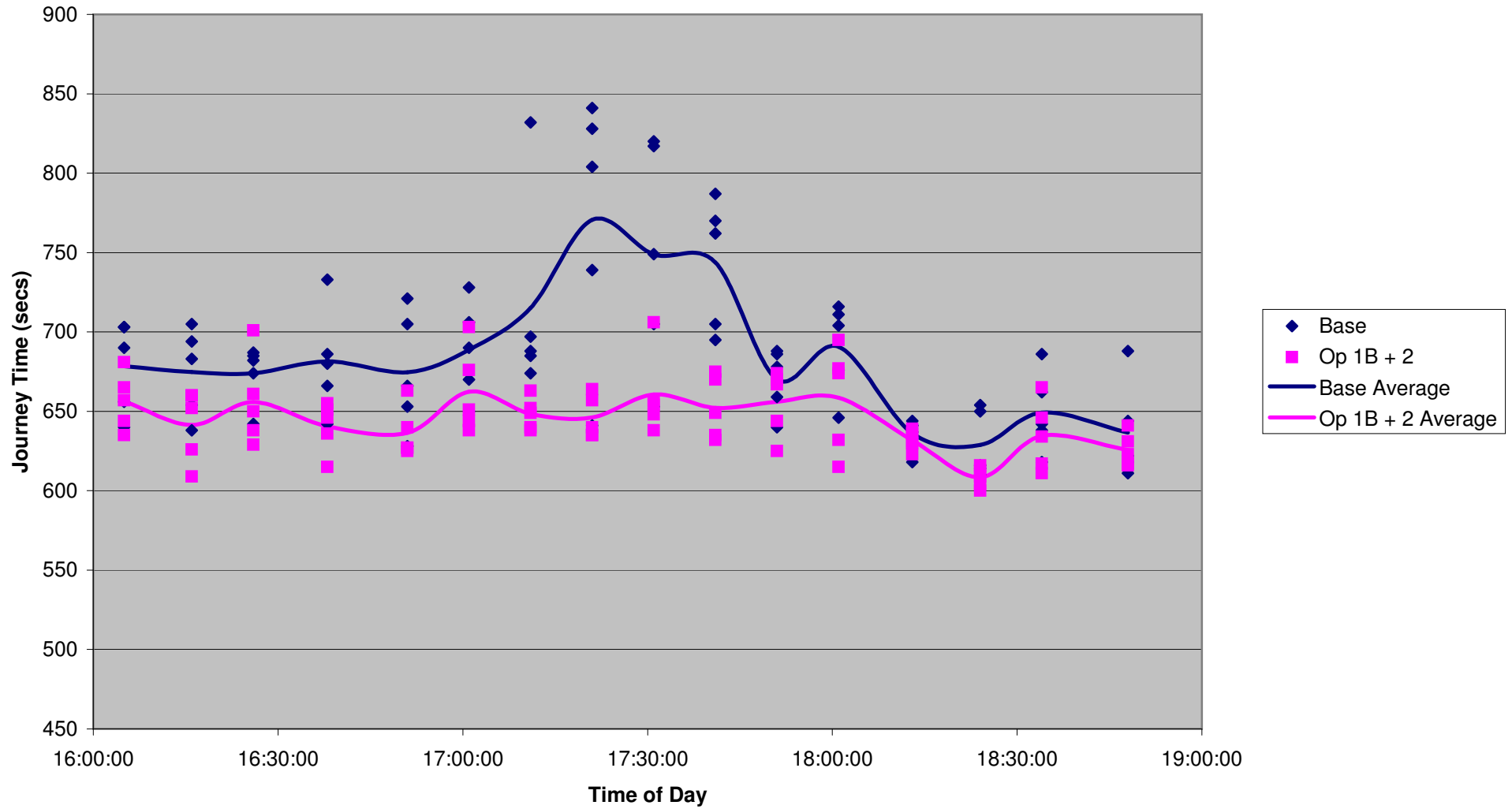
X 78 nb Evening Journey Time Variability - Base compared to Op 1B + 2
